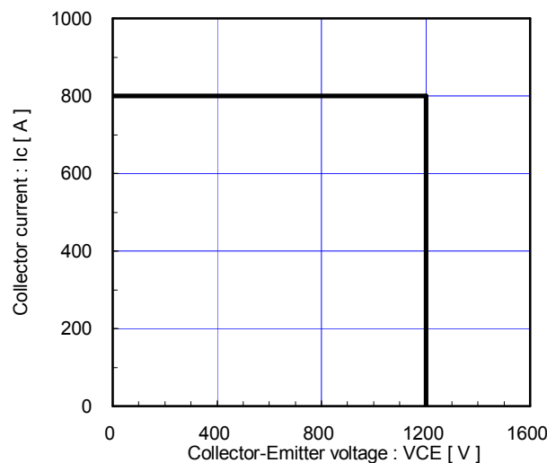
Reverse bias safe operating area (max.) +V GE =15V, -V GE ≤ 15V, R G ≥ 1.5Ω, T J ≤ 125°C
