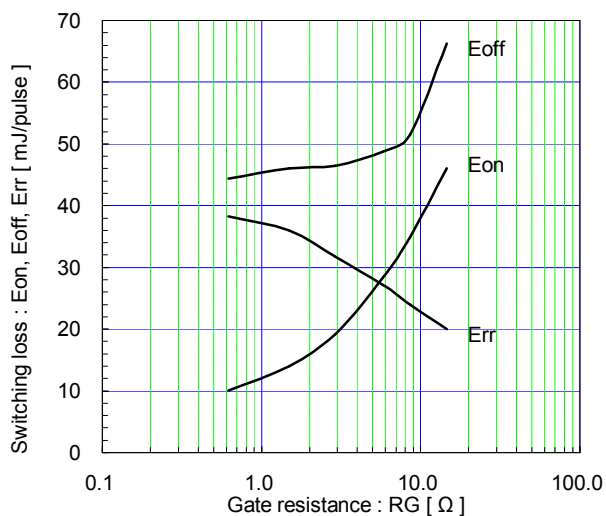
Switching loss vs. Gate resistance (typ.) V CC =600V, Ic=400A, V GE =±15V, T J =125°C
