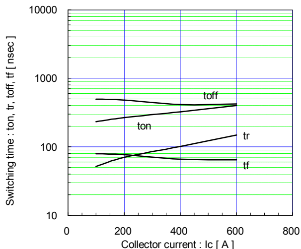
Switching time vs. Collector current (typ.) V CC =600V, V GE =±15V, R G =1.5Ω, T J =25°C
