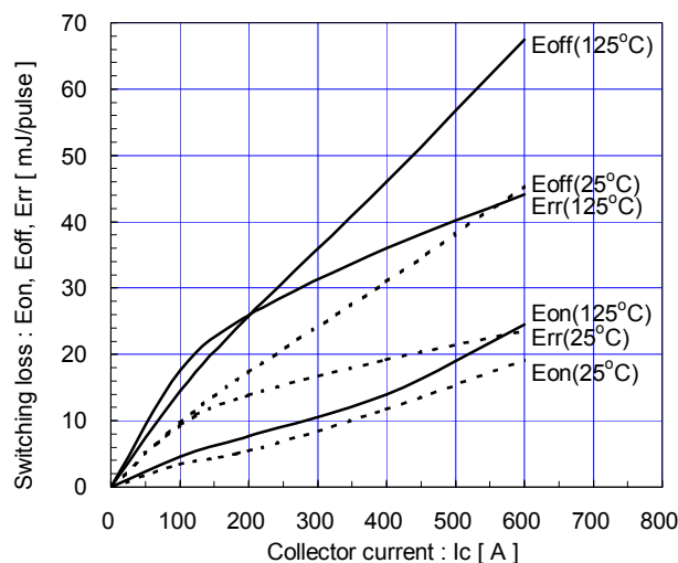
Switching loss vs. Collector current (typ.) V CC =600V, V GE =±15V, R G =1.5Ω
