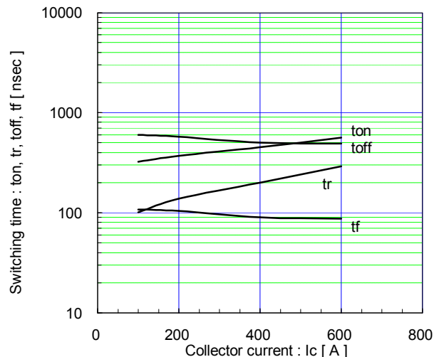
Switching time vs. Collector current (typ.) V CC =600V, V GE =±15V, R G =1.5Ω, T J =125°C
