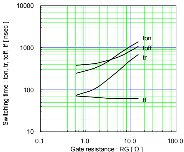
Switching time vs. Gate resistance (typ.) V CC =600V, Ic=400A, V GE =±15V, T J =25°C
