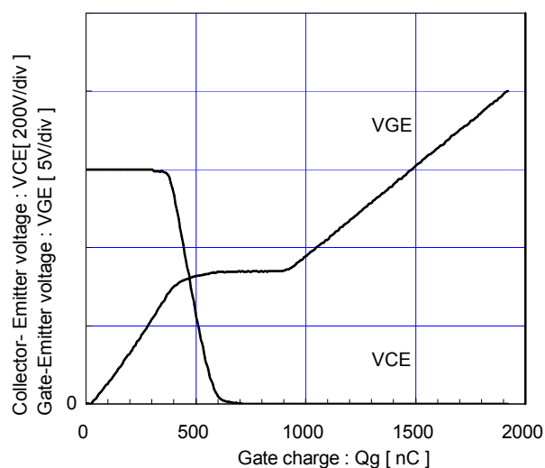
Dynamic Gate charge (typ.) Vcc=600V, Ic=400A, Tj=25°C
