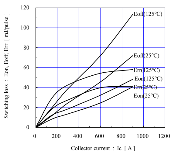
Switching loss vs. Collector current (typ.) V_{cc}=600V , V_{GE}=\pm 15V , R_g=0.6\Omega
