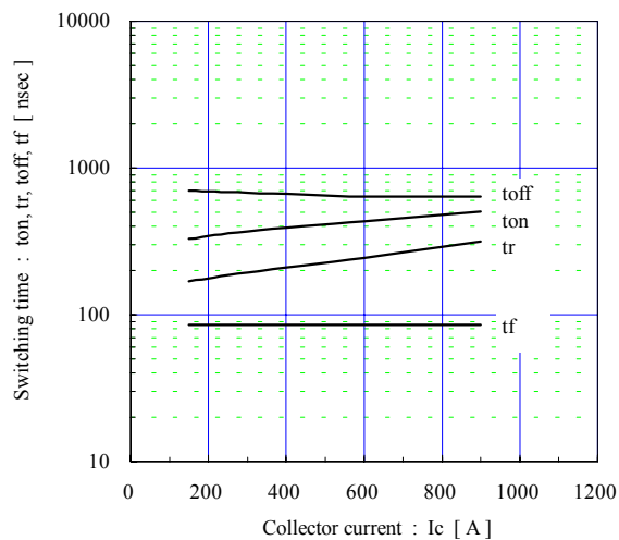
Switching time vs. Collector current (typ.) V_{cc}=600V , V_{GE}=\pm 15V , R_g=0.6\Omega , T_j=125^\circ C
