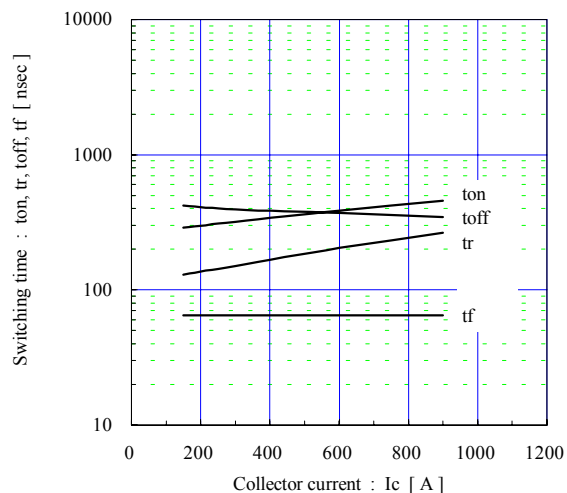
Switching time vs. Collector current (typ.) V_{cc}=600V , V_{GE}=\pm 15V , R_g=0.6\Omega , T_j=25^\circ C
