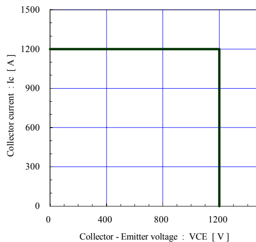
Reverse bias safe operating area (max.) +V_{GE}=15V , -V_{GE} \leq 15V , R_g \geq 0.6\Omega , T_j \leq 125^\circ C
