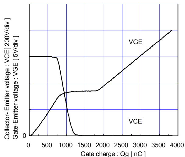
Dynamic Gate charge (typ.) Vcc=600V, Ic=800A, Tj=25°C
