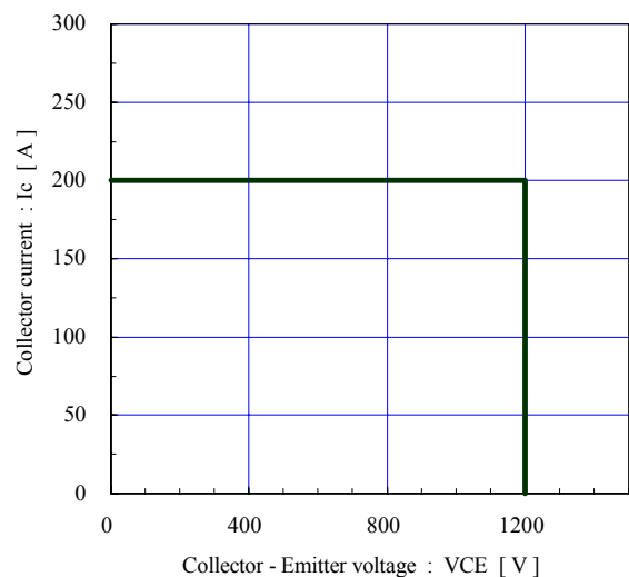
Reverse bias safe operating area (max.) +V_{GE}=15V , -V_{GE} \leq 15V , R_g \geq 5.6\Omega , T_j \leq 125^\circ C
