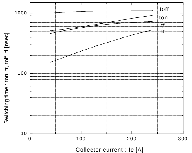
Switching time vs. Collector current V_{cc}=600\text{V} , R_G=5.6\Omega , V_{GE}=\pm 15\text{V} , T_j=125^{\circ}\text{C}
