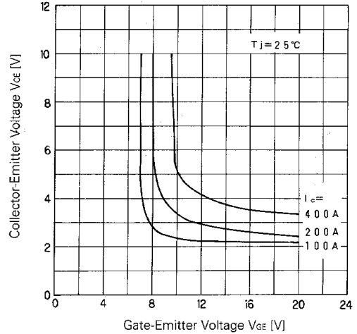
Collector-Emmitter Voltage vs. Gate-Emmitter Voltage
