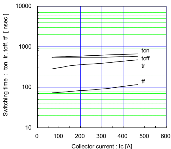
Switching time vs. Collector current (typ.) Vcc=900V, VGE=±15V, Rg=1.5Ω, Tj= 25°C
