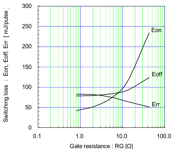
Switching loss vs. Gate resistance (typ.) Vcc=900V, Ic=300A, VGE=±15V, Tj= 125°C
