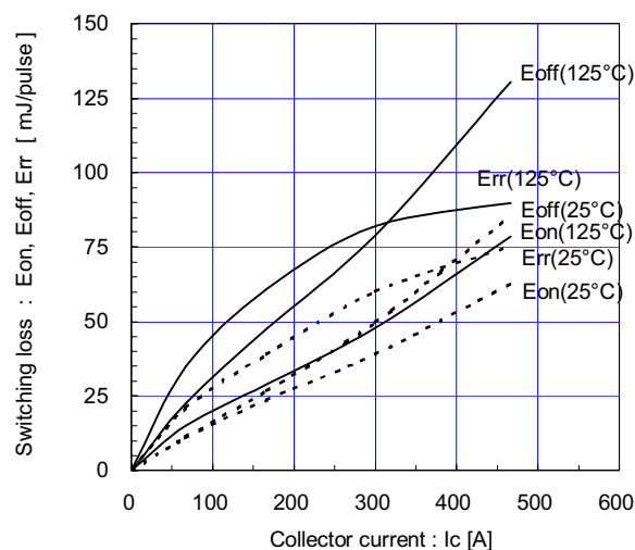
Switching loss vs. Collector current (typ.) Vcc=900V, VGE=±15V, Rg=1.5Ω
