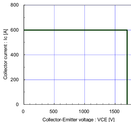
Reverse bias safe operating area (max.) +VGE=15V, -VGE ≤ 15V, Rg ≥ 1.5Ω, Tj ≤ 125°C
