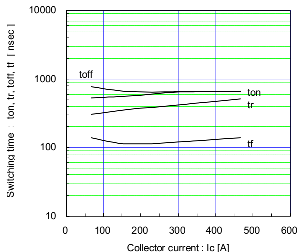
Switching time vs. Collector current (typ.) Vcc=900V, VGE=±15V, Rg=1.5Ω, Tj=125°C
