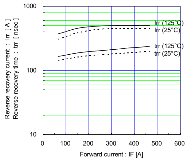
Reverse recovery characteristics (typ.) Vcc=900V, VGE=±15V, Rg=1.5Ω
