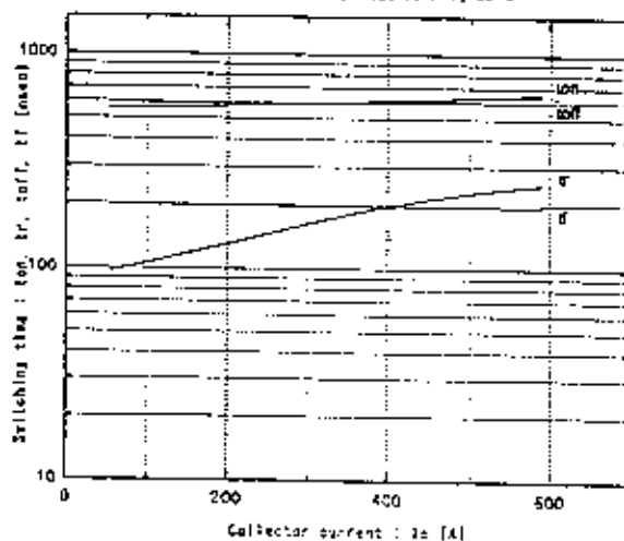
Switching time vs. Collector current Vce=300V, RθJA=10, VGE=15V, Tj=25°C
