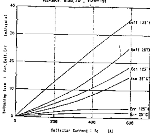
Switching loss vs. Collector current V_{CE}=100V , R_{GD}=7\Omega , V_{BE}=+15V
