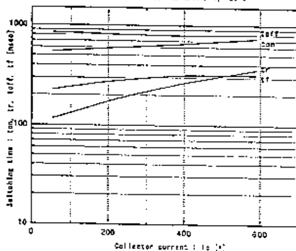
Switching time vs. Collector current Vce=300V, RθJA=10, VGE=15V, Tj=125°C
