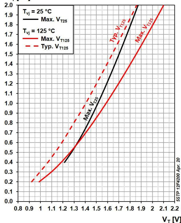
Fig. 2 On-state voltage characteristics
