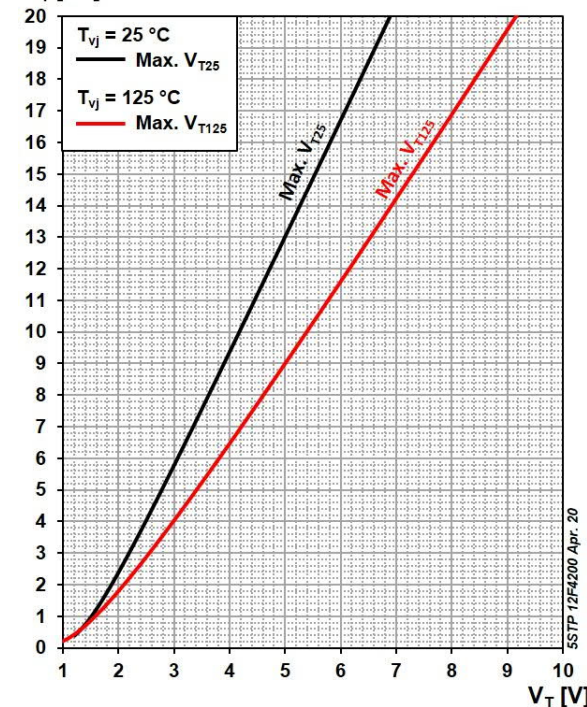
Fig. 3 On-state voltage characteristics
