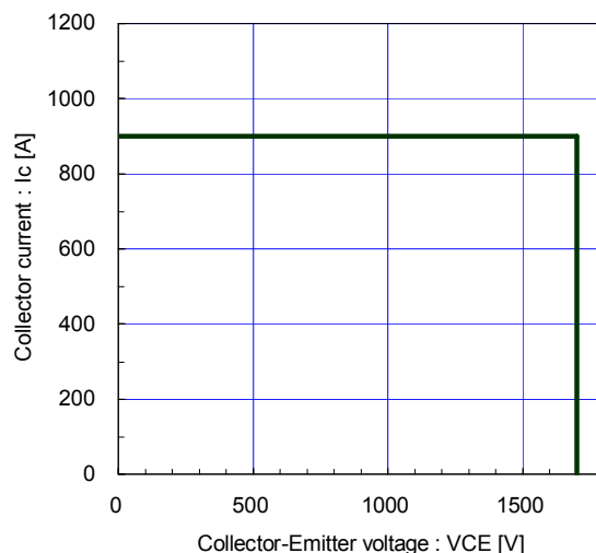
Reverse bias safe operating area (max.) +V_{GE}=15V , -V_{GE} \leq 15V , R_g \geq 1.1\Omega , T_j \leq 125^\circ C Stray inductance \leq 100nH
