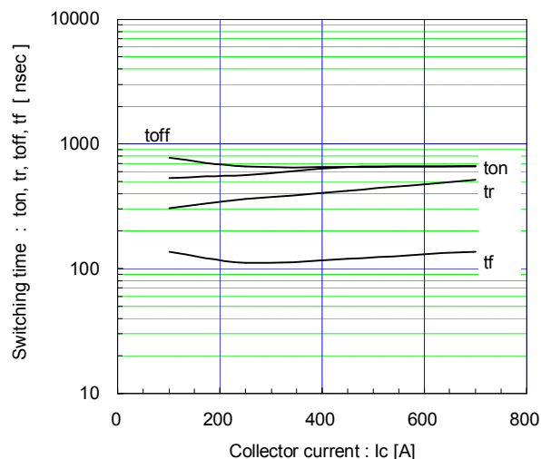
Switching time vs. Collector current (typ.) V_{cc}=900V , V_{GE}=\pm 15V , R_g=1.1\Omega , T_j=125^\circ C
