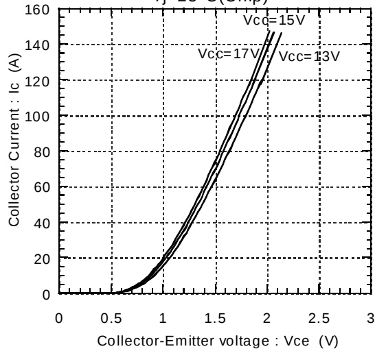
Collector current vs. Collector-Emitter voltage T_j=25^{\circ}\text{C}(\text{Chip})
