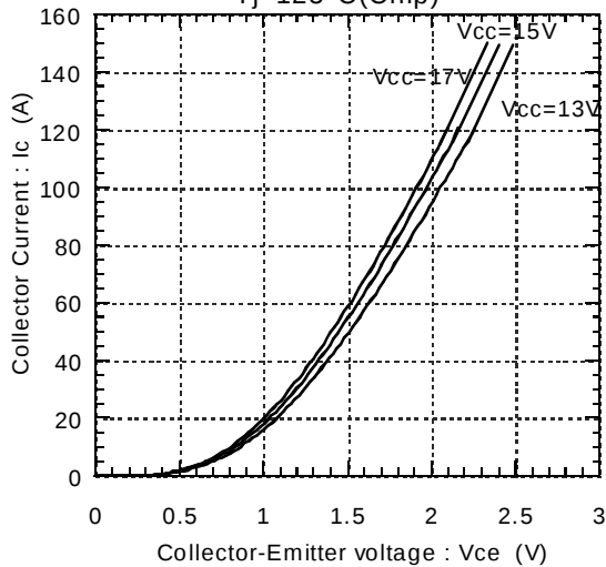
Collector current vs. Collector-Emitter voltage T_j=125^{\circ}\text{C}(\text{Chip})
