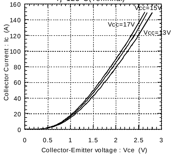
Collector current vs. Collector-Emitter voltage T_j=125^{\circ}\text{C}(\text{Terminal})
