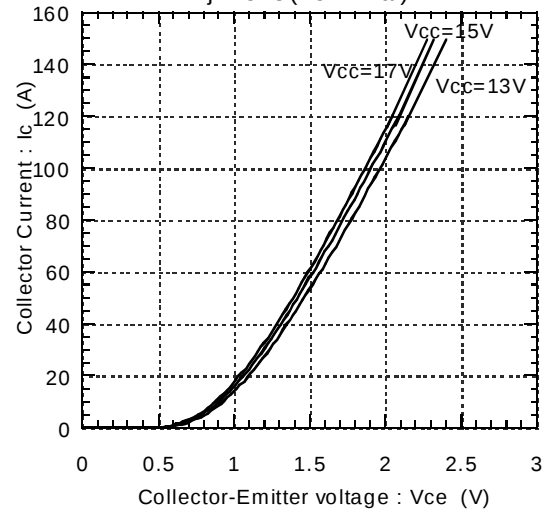
Collector current vs. Collector-Emitter voltage T_j=25^{\circ}\text{C}(\text{Terminal})
