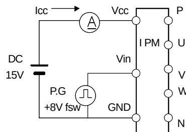
Figure 7. Icc Test Circuit
