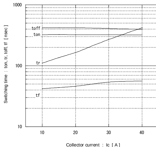
[ Inverter ] Switching time vs. Collector current (typ.) V_{CC}=300V , V_{GE}=+15V , R_g=150\Omega , T_j=125^\circ C
