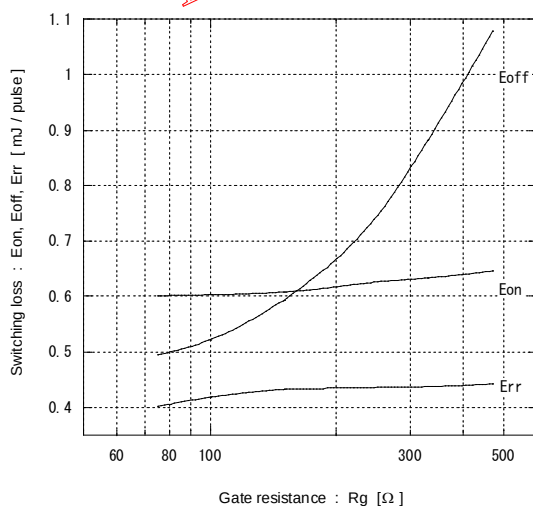
[ Inverter ] Switching loss vs. Gate resistance (typ.) V_{CC}=300V , I_c=20A , V_{GE}=+15V , T_j=125^\circ C
