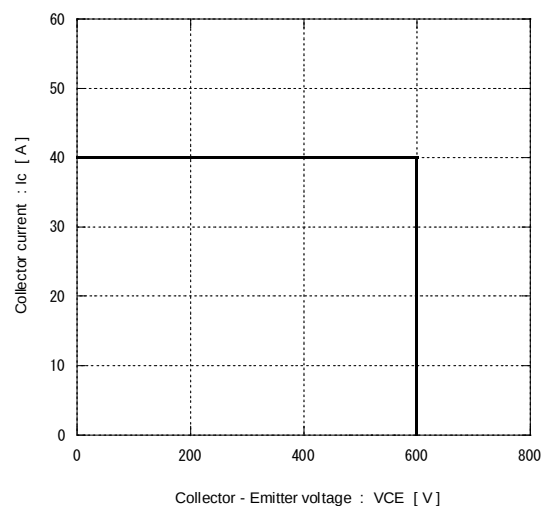
[ Inverter ] Reverse bias safe operating area (max) +V_{GE}=15V , -V_{GE}\leq -15V , R_g\geq 150\Omega , T_j\leq 125^\circ C
