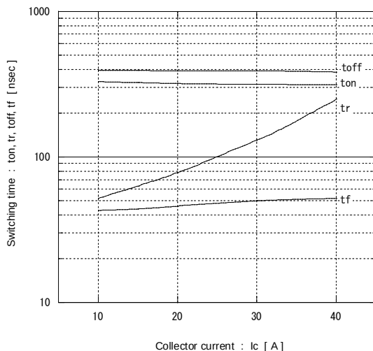
[ Inverter ] Switching time vs. Collector current (typ.) V_{CC}=300V , V_{GE}=+15V , R_g=150\Omega , T_j=25^\circ C
