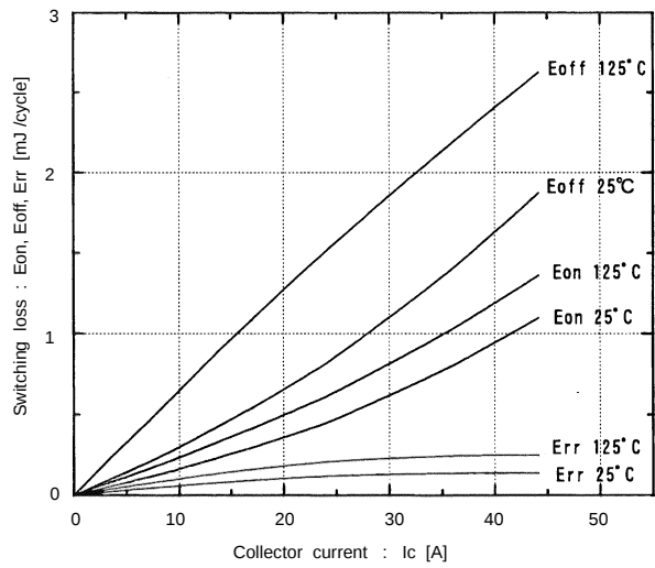
Switching loss vs. Collector current Vcc=300V, RG=82 ohm, VGE=±15V
