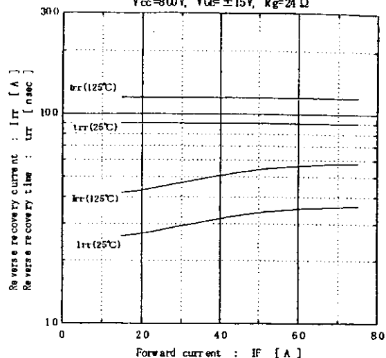
[ Inverter ] Reverse recovery characteristics (typ.) V_{CC}=800V , V_{GE}=\pm 15V , R_g=24\Omega
