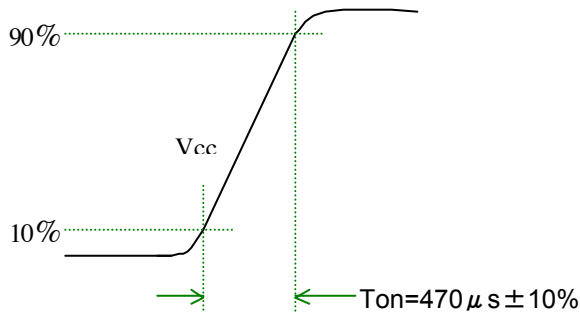
Sequence of Power-on/off and signal-on/off
