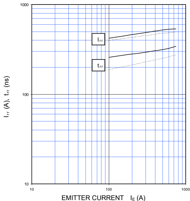
FREE WHEELING DIODE REVERSE RECOVERY CHARACTERISTICS (TYPICAL) V_{CC}=1000\text{ V} , V_{GE}=\pm 15\text{ V} , R_G=2.0\text{ }\Omega , INDUCTIVE LOAD —: T_j=150\text{ }^\circ\text{C} , - - - -: T_j=125\text{ }^\circ\text{C}
