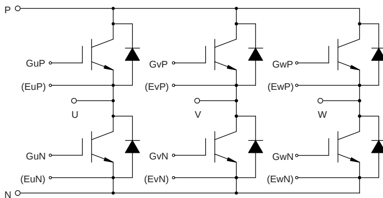
Outline Drawing and Circuit Diagram
