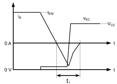
t_{rr} , Q_{rr} test waveform
