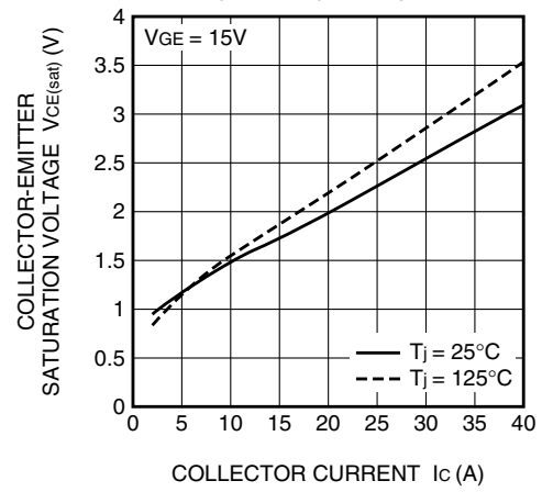
COLLECTOR-EMITTER SATURATION VOLTAGE CHARACTERISTICS (TYPICAL) Brake part
