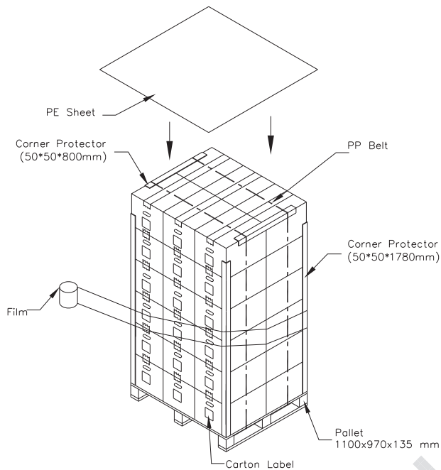
Figure. 9-2 Packing method
