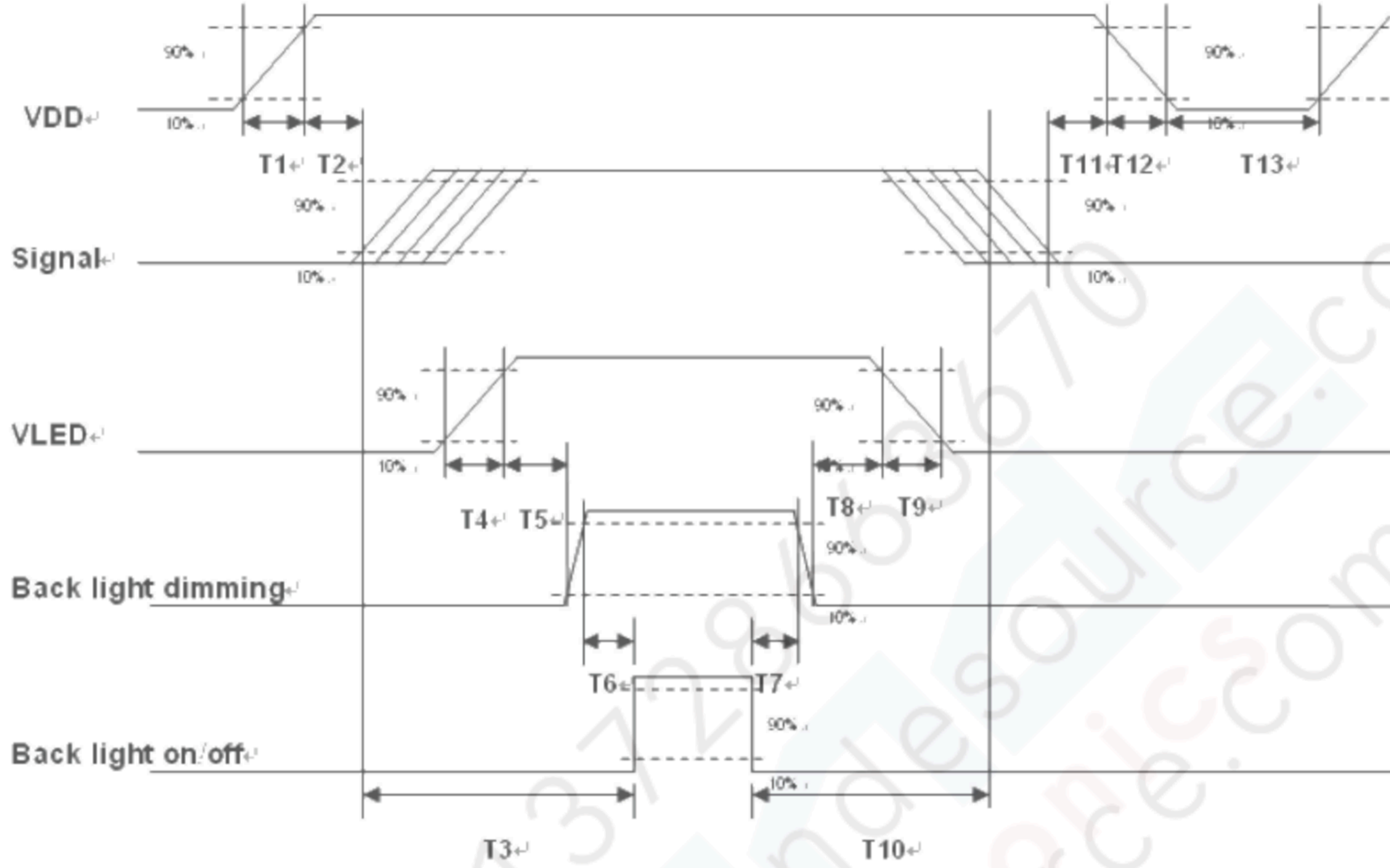
Power ON/OFF sequence timing
