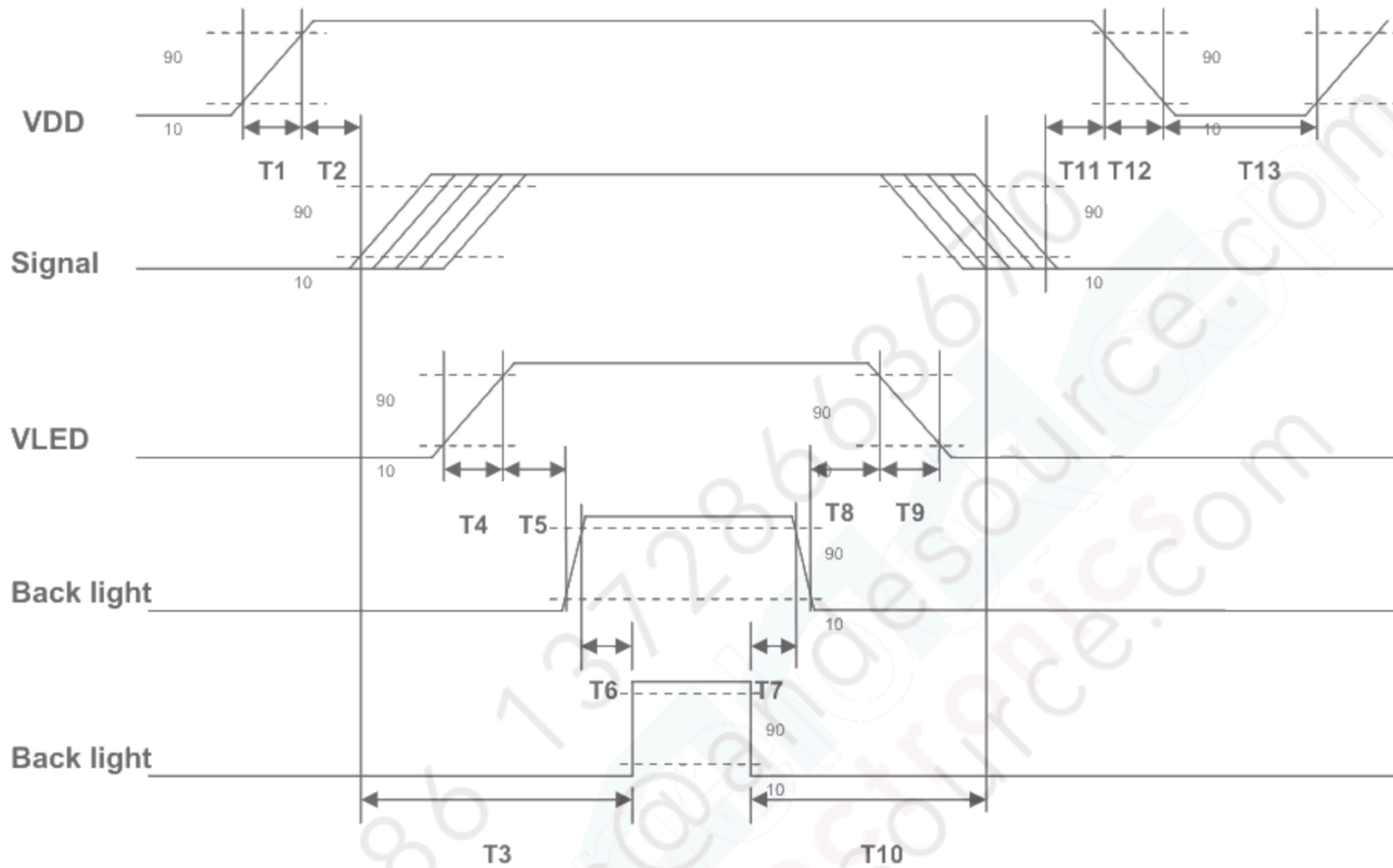
Power Sequence Timing
