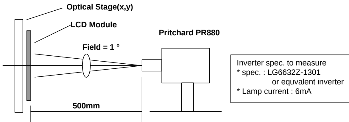
FIG. 1 Optical Characteristic Measurement method
