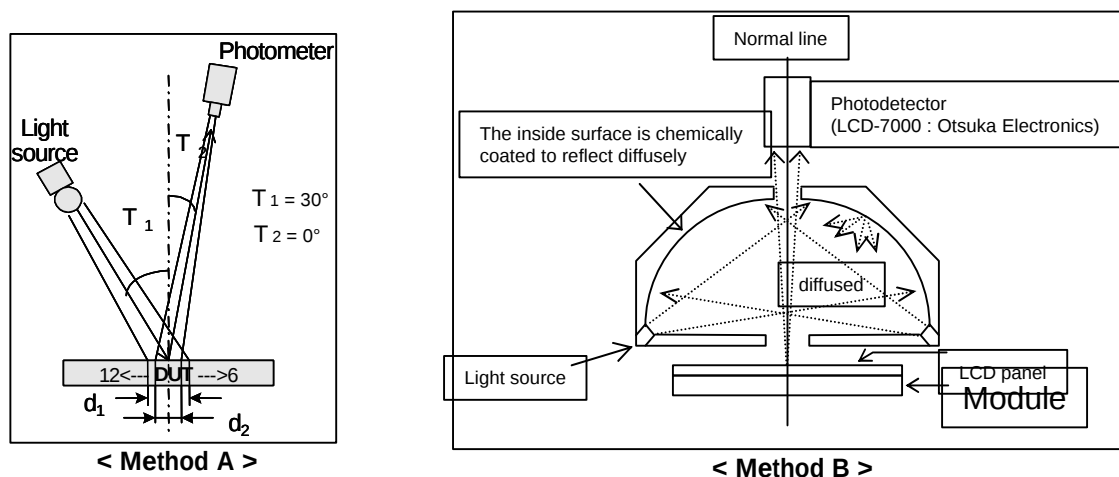
FIG. 2 Optical Characteristic Measurement methods
