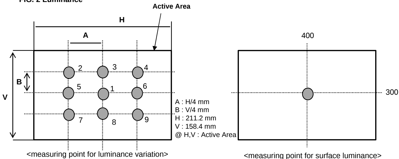
FIG. 2 Luminance
