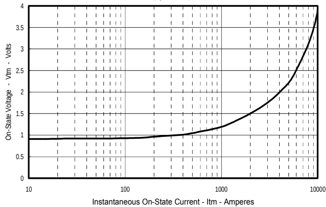
Typical On-State Forward Voltage Drop ( T_J = 125^\circ\text{C} )
