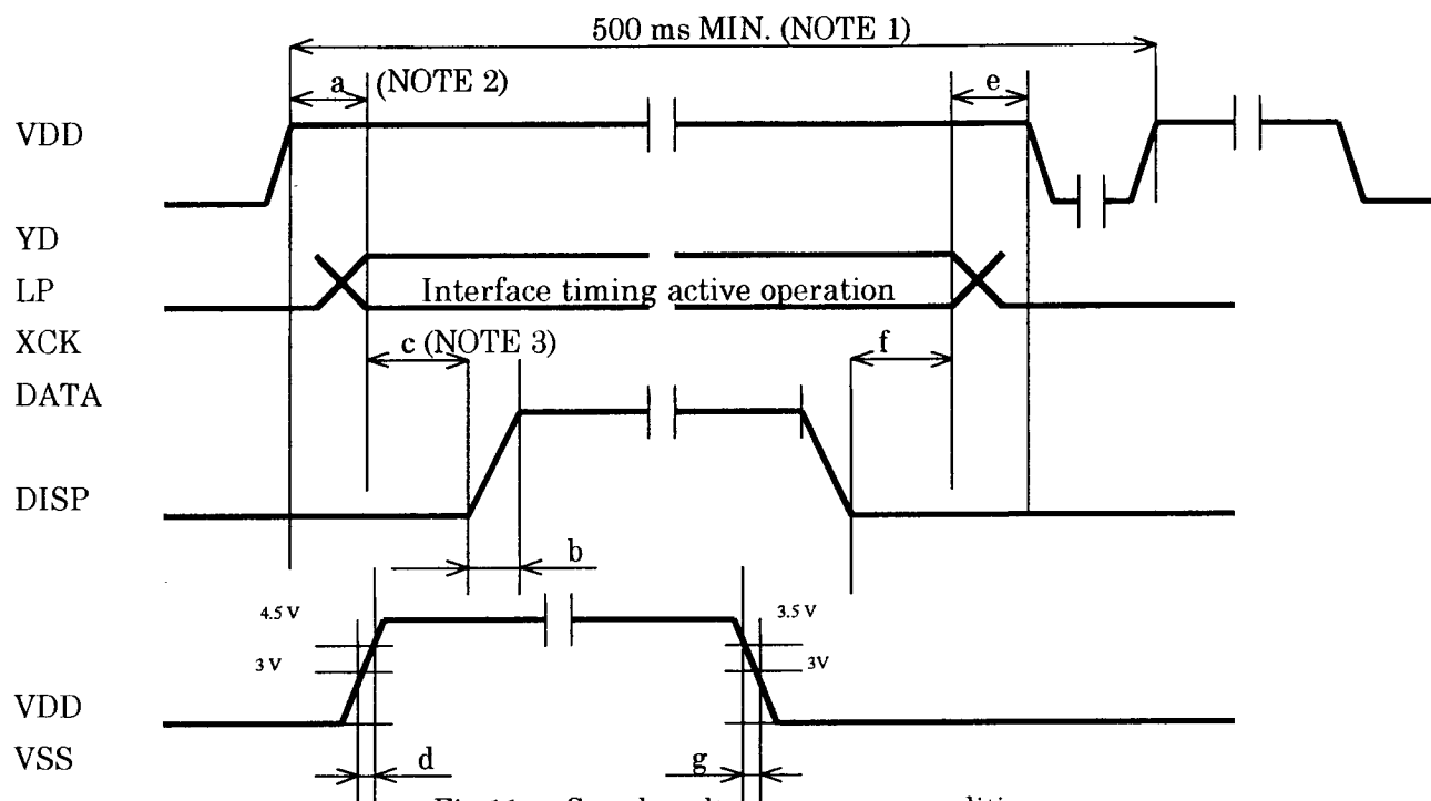
Fig.11 Supply voltage sequence condition
