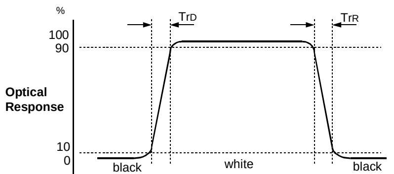
FIG. 3 Response Time
