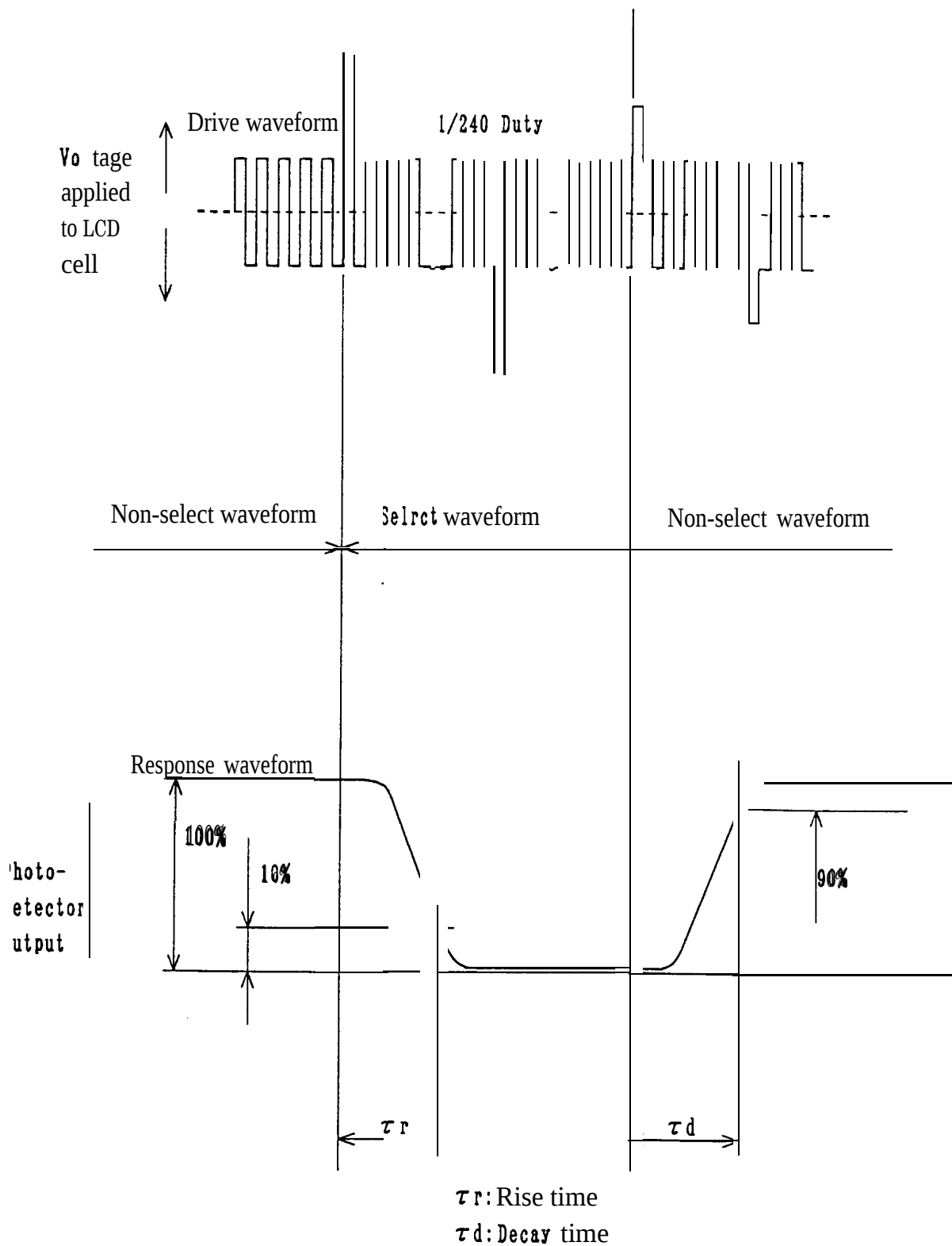
Fig. 6 Definition of response Time
