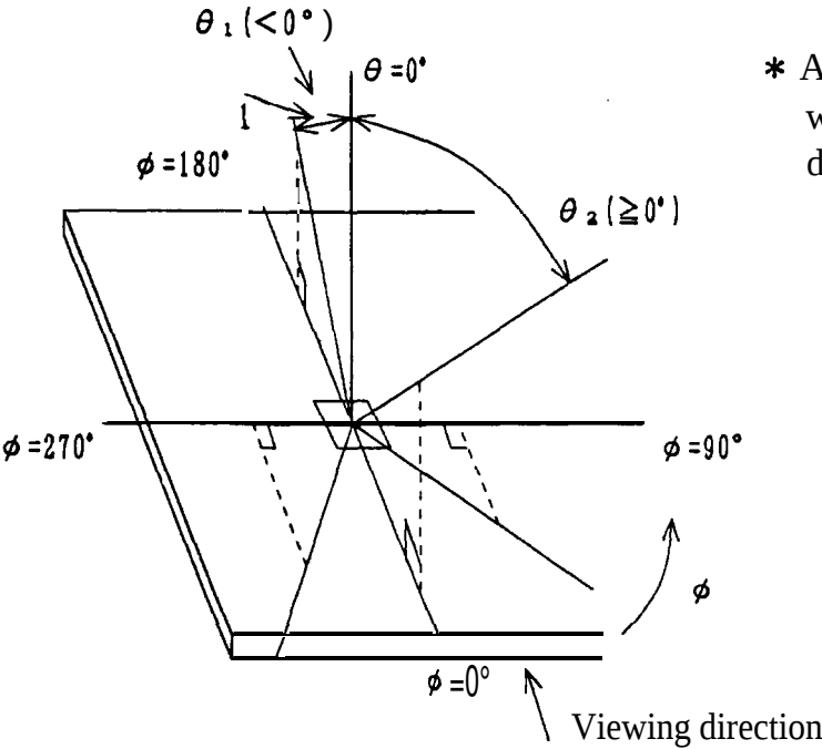
Fig. 4 Definition of Viewing Angle
