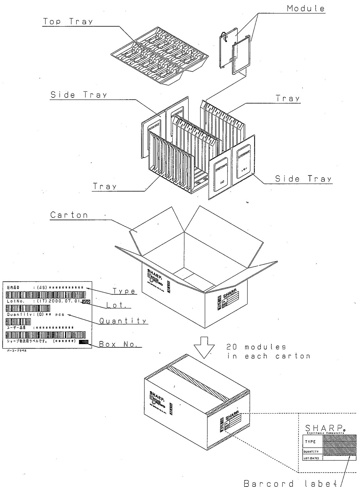
Fig 3 PACKING FORM
