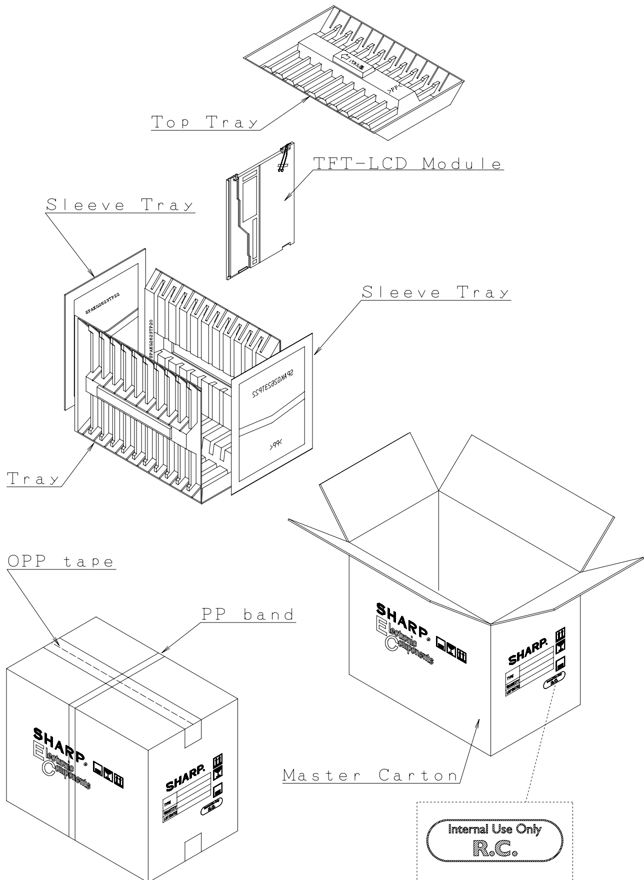
Fig2. Packing Form
