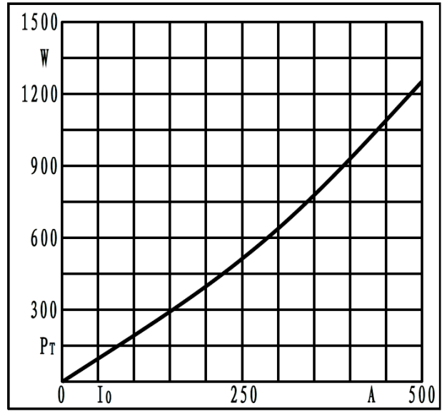
Fig2. Power dissipation
