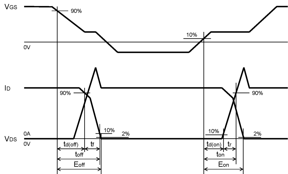
Fig. 7.3 Timing Chart (MOSFET part)
