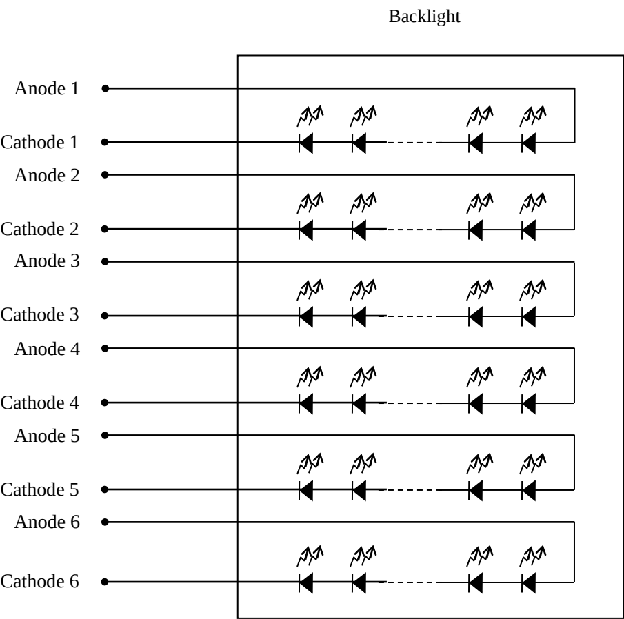
Note3: Backlight detail
