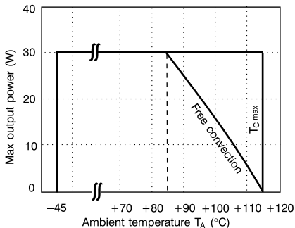
Power derating
