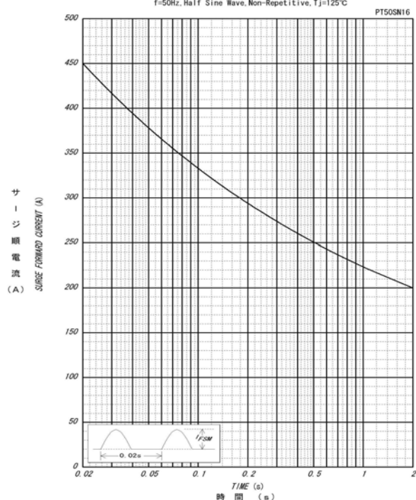
サージ順電流定格 SURGE CURRENT RATINGS f=50Hz, Half Sine Wave, Non-Repetitive, Tj=125°C
