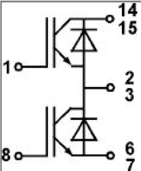
Case T 32 GB
