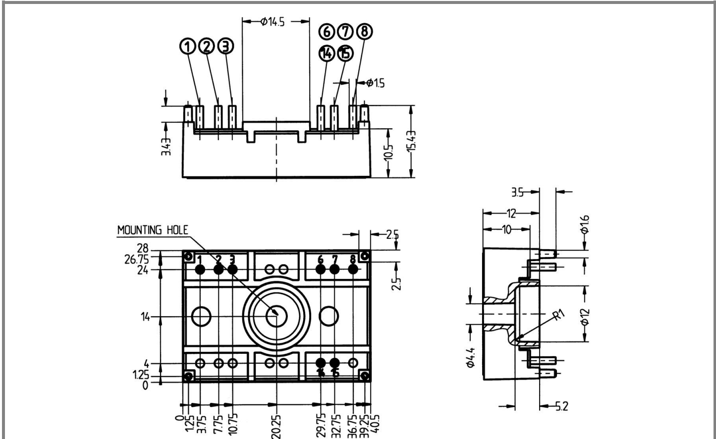
Case T32 (Suggested hole diameter for solder pins and plastic mounting pins: 2mm)
