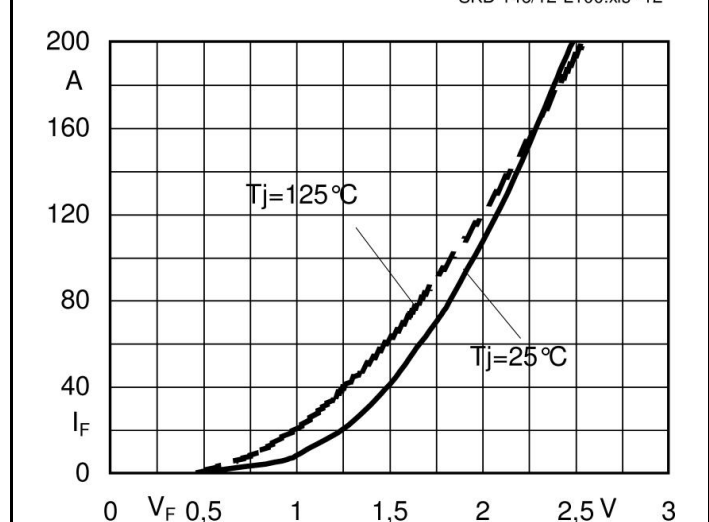
Fig. 10 Diode forward characteristic
