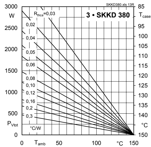
Fig. 13R Power dissipation of three modules vs. case temp.
