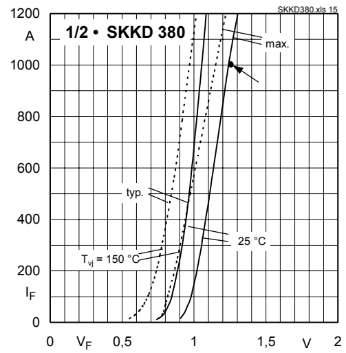
Fig. 15 Forward characteristics
