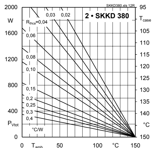
Fig. 12R Power dissipation of two modules vs. case temp.
