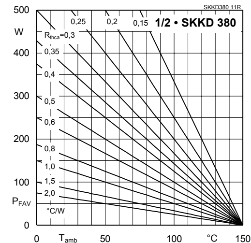
Fig. 11R Power dissipation per diode vs. ambient temp.
