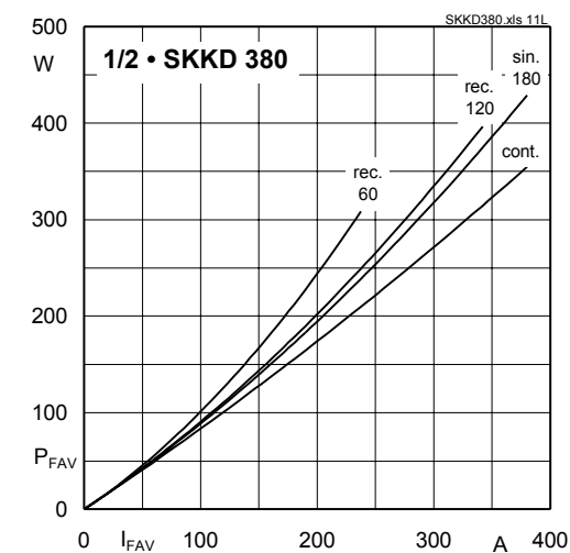
Fig. 11L Power dissipation per diode vs. on-state current
