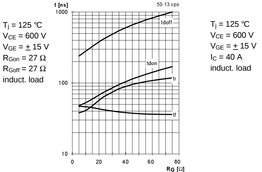
Fig. 16 Typ. switching times vs. gate resistor R_G
