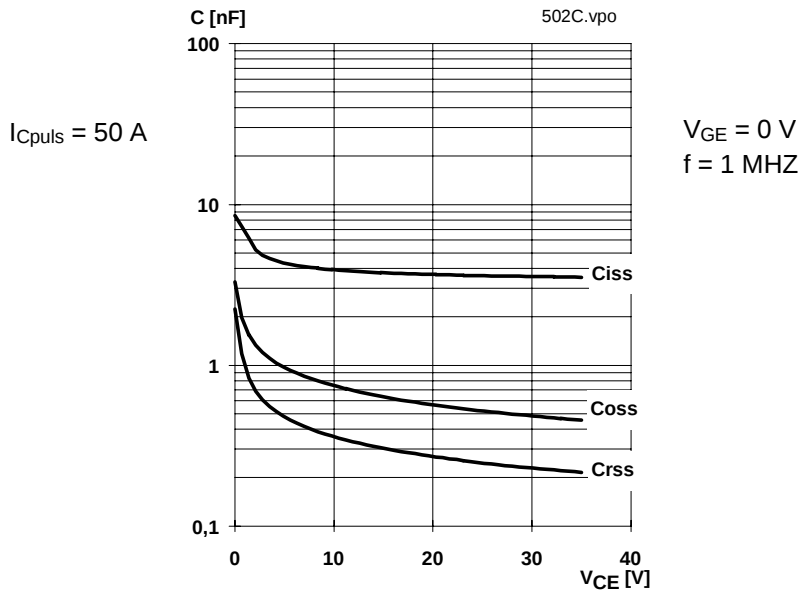
Fig. 14 Typ. capacitances vs. V_{CE}
