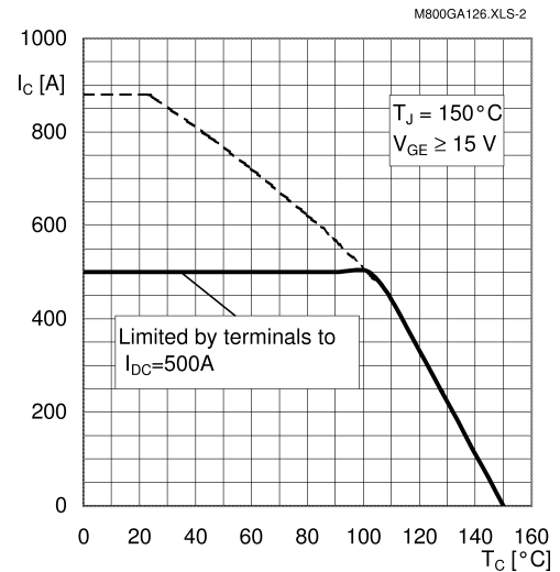
Fig. 2: Rated current vs. temperature I_C = f(T_C)
