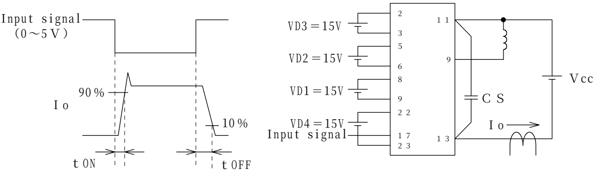
Fig 6 : Switching Time
