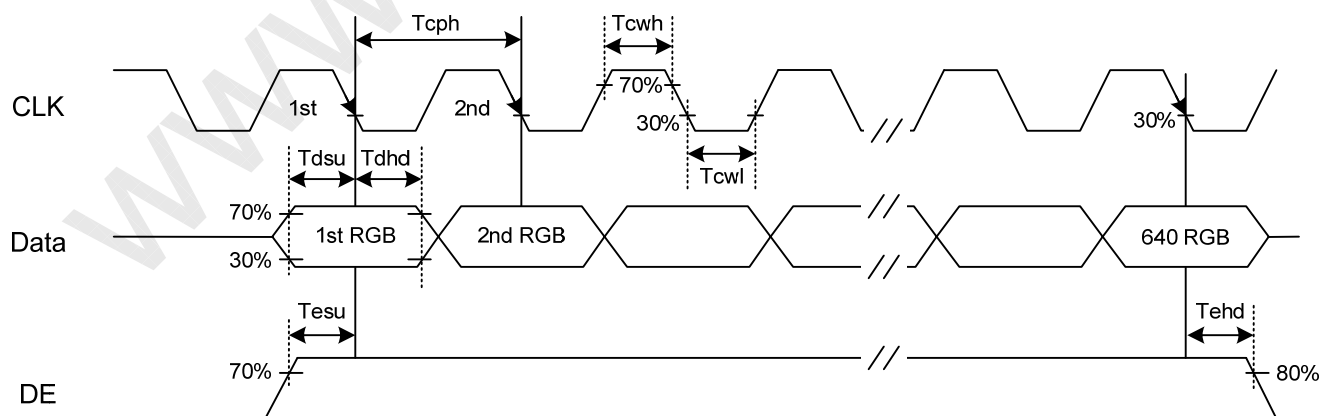
Fig. 9.3 Setup &amp; Hold Time
